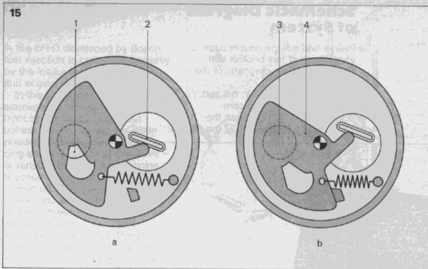
Fig. 15 Diagrams showing operation of the auxiliary-air device with external heating 1 Opening for auxiliary air 2 Bimetallic strip with heating winding 3 Cross-section of bypass channel partly open in drawing "a", closed in drawing "b" 4 Blocking plate a Bypass channel partly open b Bypass channel closed (engine at normal operating temperature)
