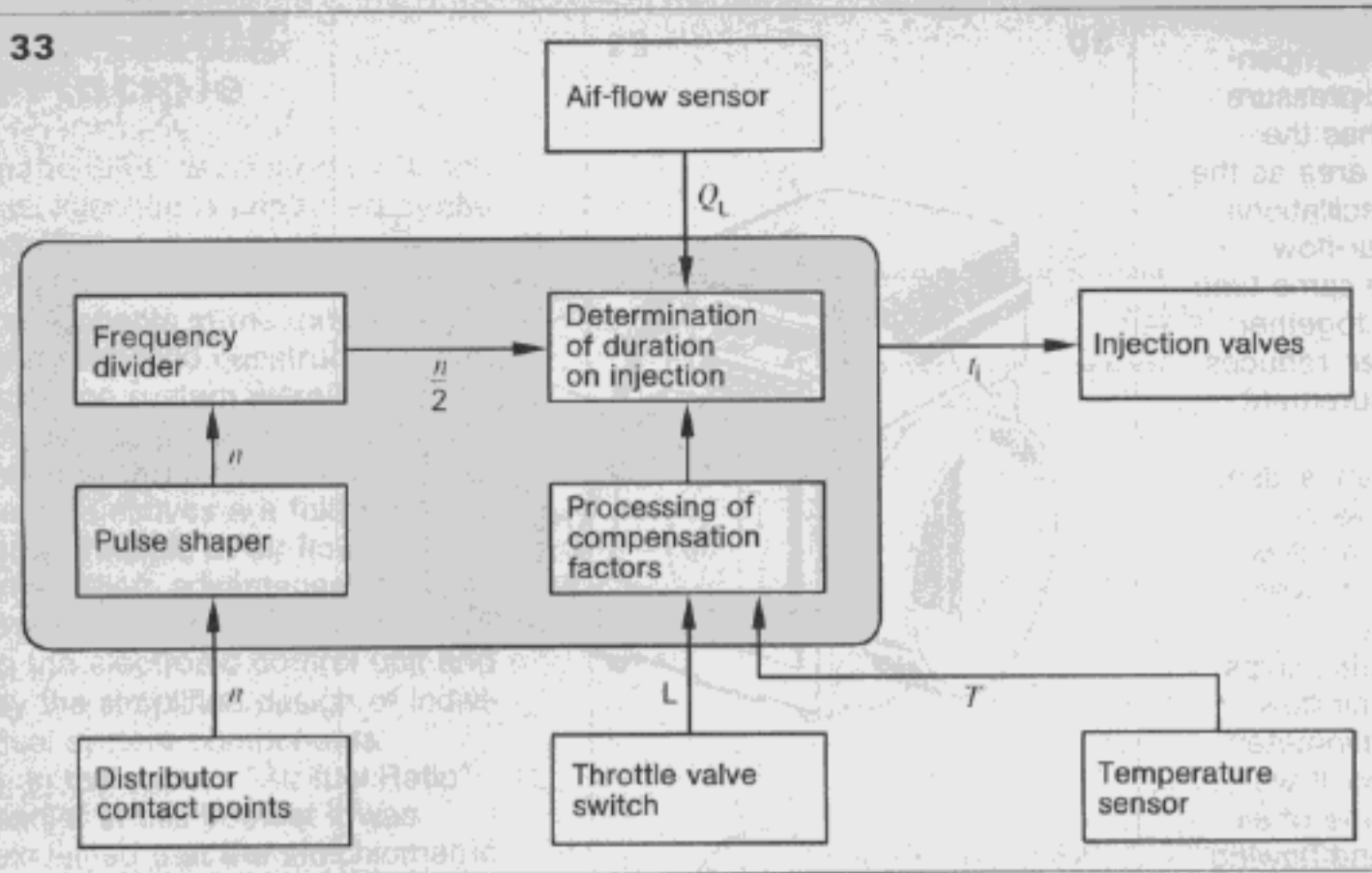
Fig. 33 Block operating diagram of the EFI-L Signals for: n Rotational speed Q_L Amount of air T Temperature t_i Duration of injection L Idle, full-load
