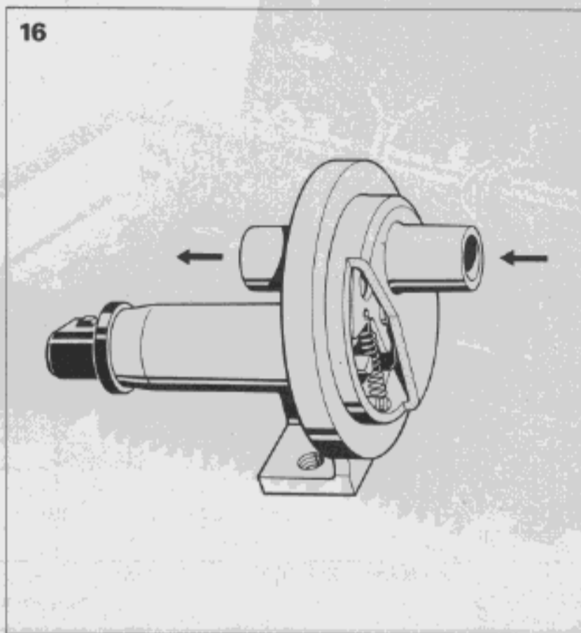
Fig. 16 Auxiliary-air device with external heating
