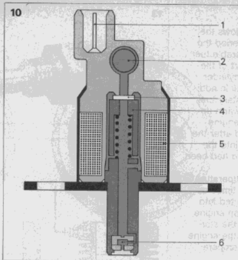
Fig. 10 Start valve
