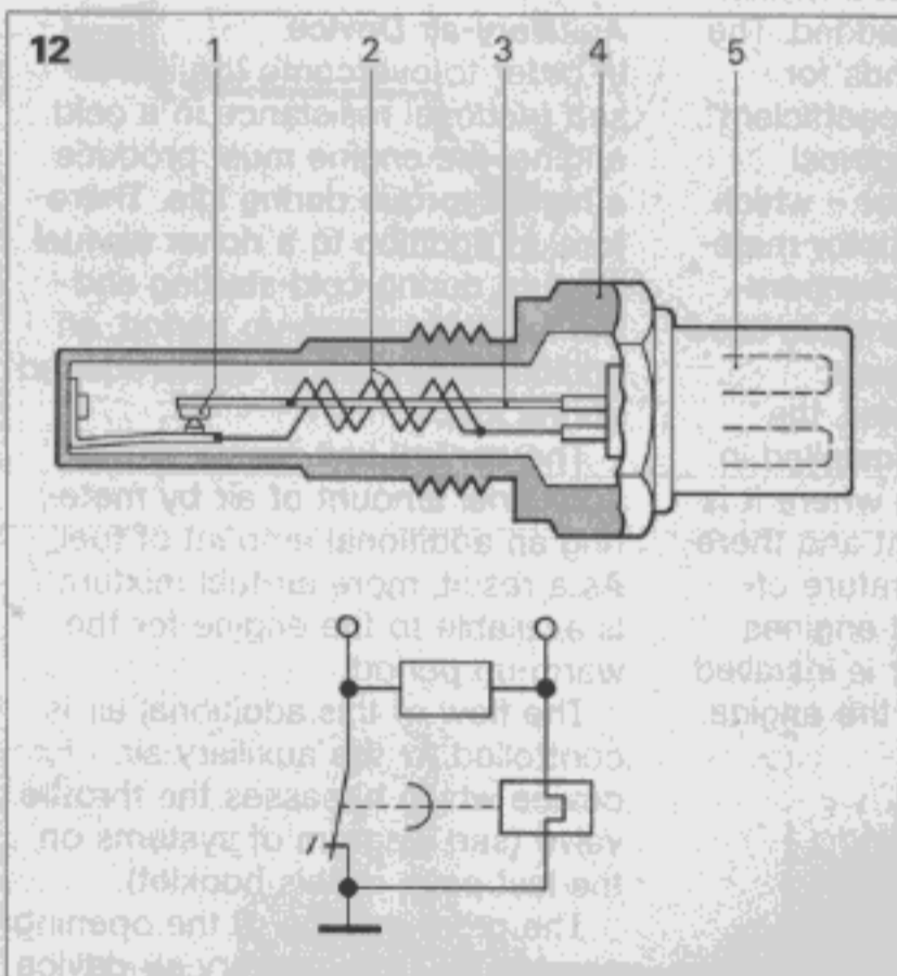
Fig. 12 Cross-sectional drawing of the thermo-time switch
