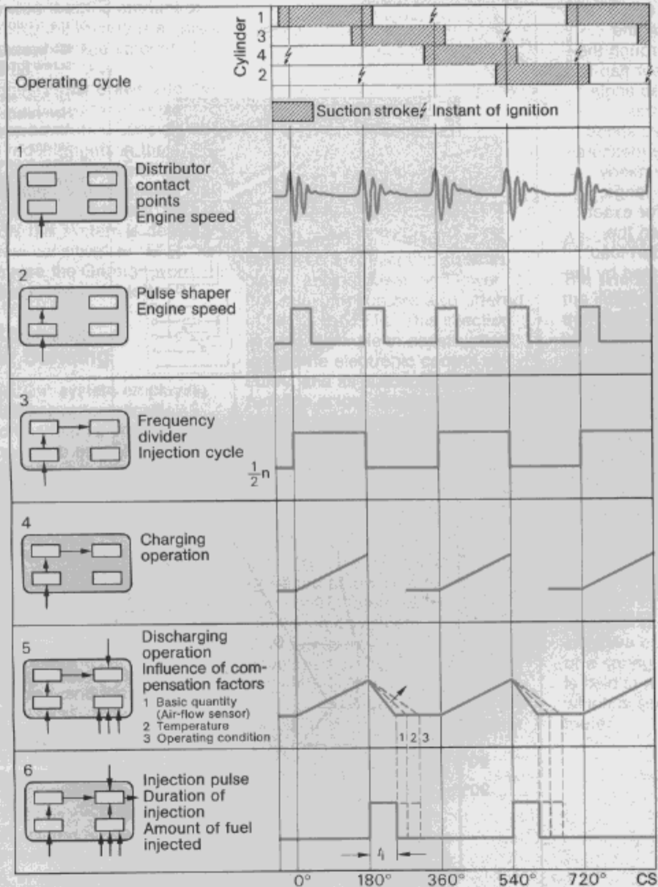
Fig. 34 Diagram of pulses in EFI-L
