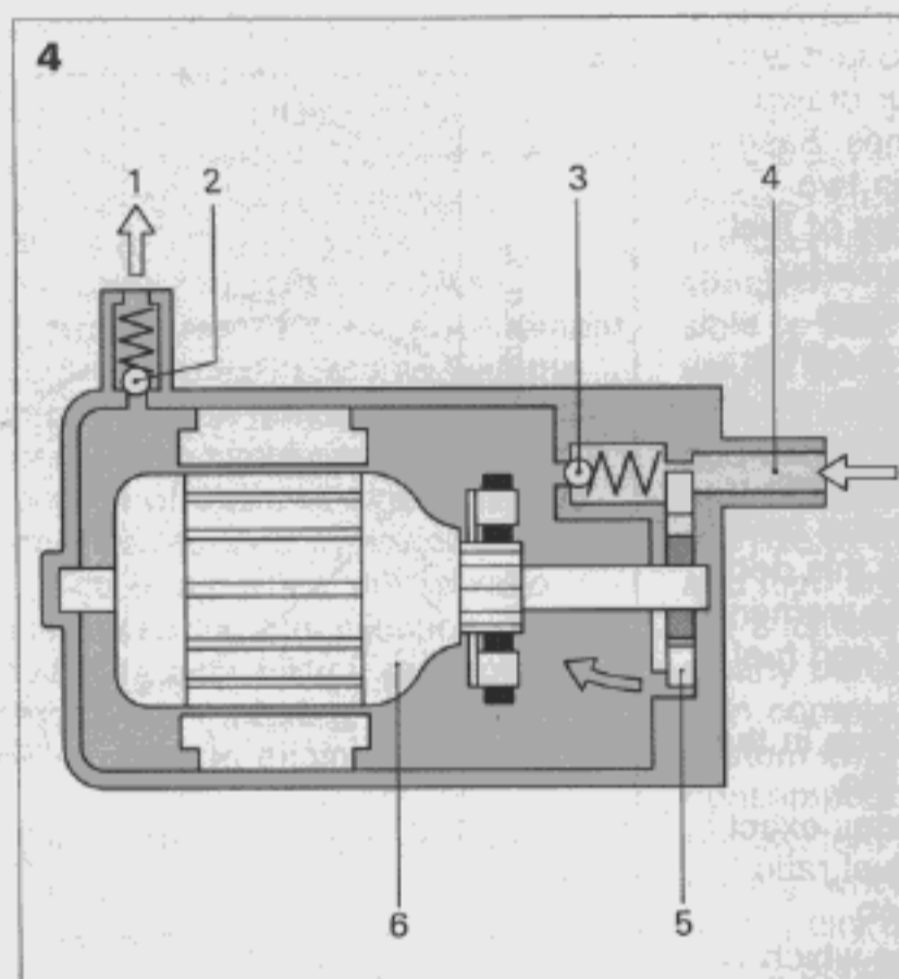
Fig. 4 Electric fuel pump
