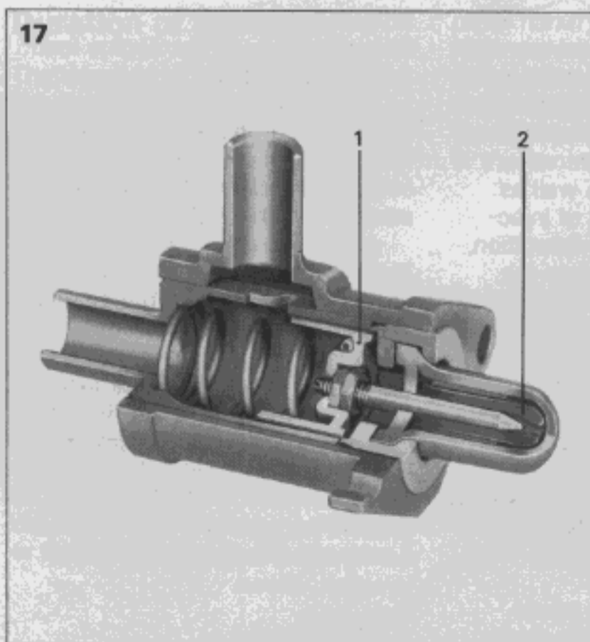
Fig. 17 Auxiliary-air device with expansion element 1 Piston 2 Expansion element
