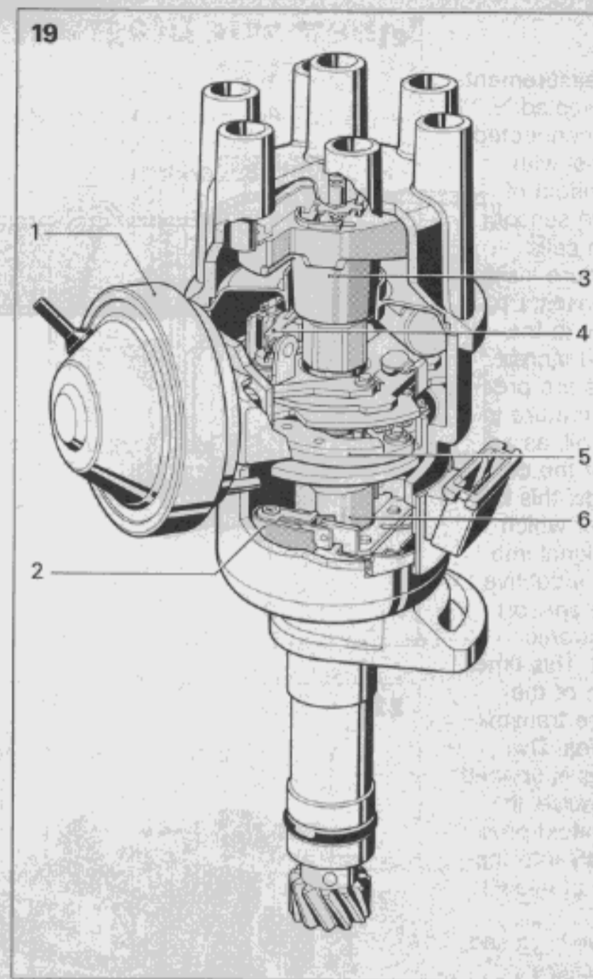
Fig. 19 Ignition distributor with trigger contacts (6-cylinder engine)
