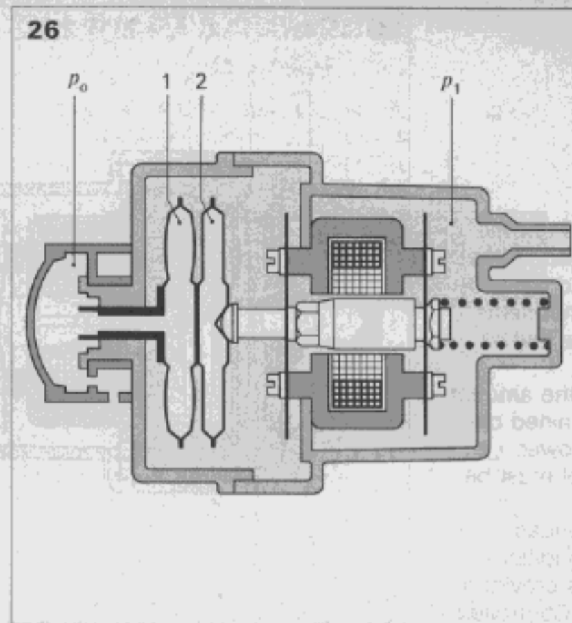
Fig. 26 Pressure sensor without diaphragm for the full-load enrichment, with altitude compensation
