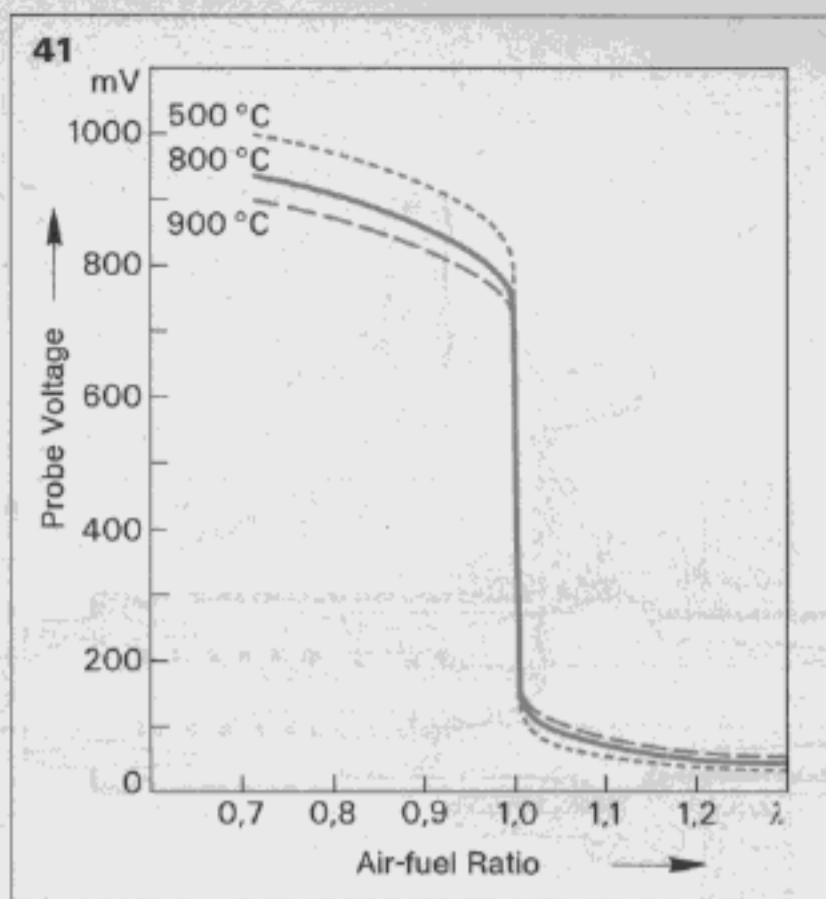
Fig. 41 Operating characteristic of the Lambda probe
