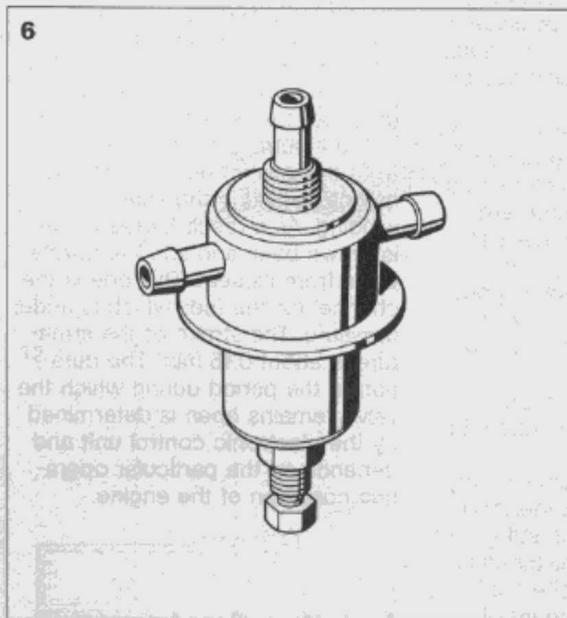
Fig. 6 Fuel-pressure regulator (EFI-D)
