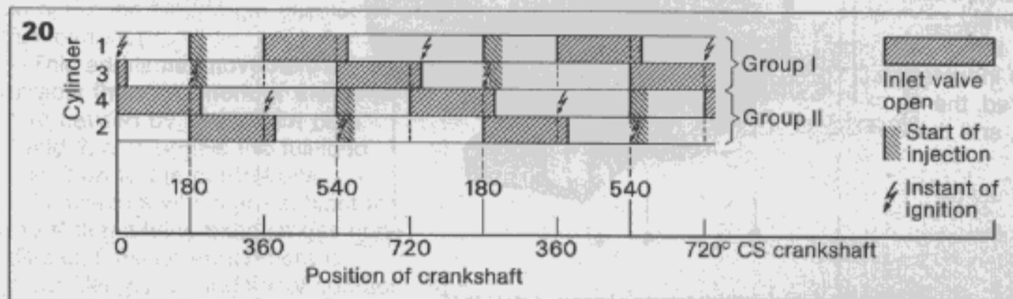
Fig. 20 Fuel injection timing diagram (EFI-D)
