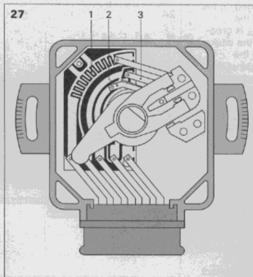
Fig. 27 Throttle valve switch
