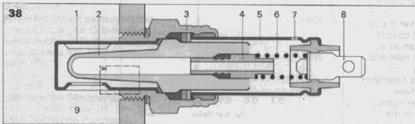
Fig. 38 Cross-sectional drawing of the Lambda probe
