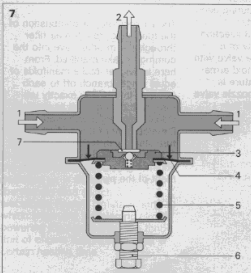
Fig. 7 Cross-sectional drawing of the fuel-pressure regulator
