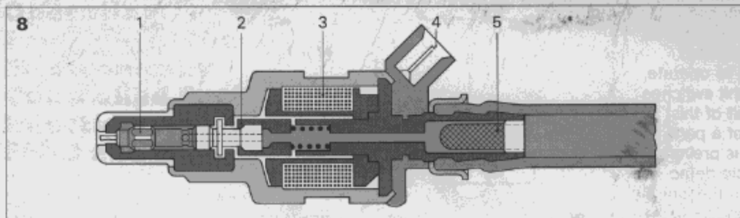
Fig. 8 Cross-sectional drawing of the injection valve
